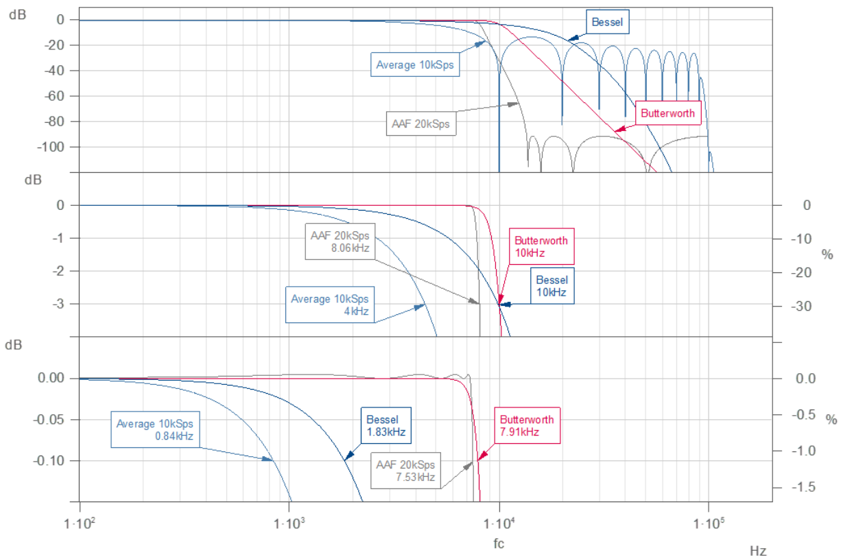
Fig. 18: Comparison of different filter characteristics for low-pass filters ( f_{s\ prim} = 200\ kSps )
